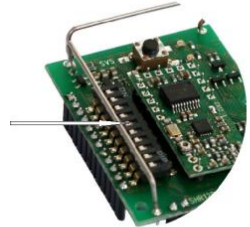
DIP-Schalter 5 in Pos. OFF = Frequenz 1 DIP-Schalter 5 in Pos. ON = Frequenz 2
